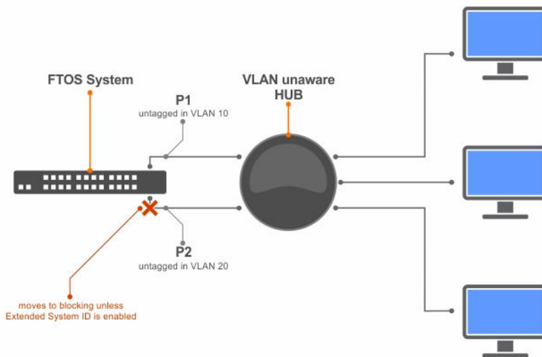
Figure 98. PVST+ with Extend System ID
